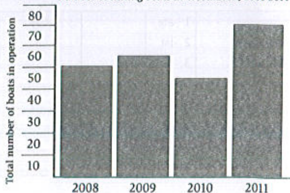
Number of fishing boats in Westhaven, 2008-2011
