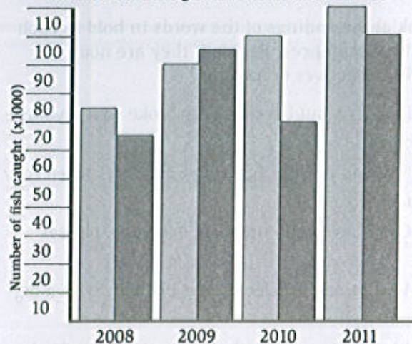
Number of fish caught near Westhaven, 2008-2011
